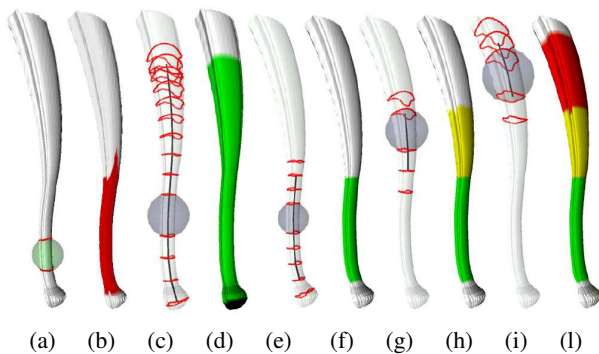
Figure 10: (a) Initial level of detail, (b) limb-region, (c) tube growing in non-strict mode, and (d) tube extraction. In (e) tube growing from the same limb-vertices in strict mode, (f) the extracted tube, (g), (h) (i) next iterations, (l) achieved segmentation at the chosen scale.
